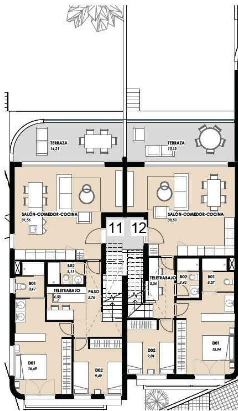
VIVIENDA 11-12_PLANTA PRIMERA/ APARTMENT 11-12_TOP FLOOR 1 : 100
