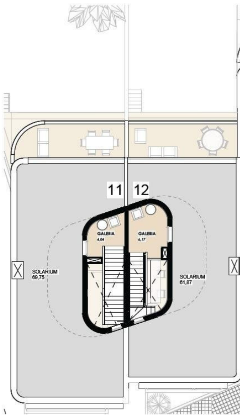
VIVIENDA 11-12_SOLARIUM/ APARTMENT 11-12_SOLARIUM 1 : 100
