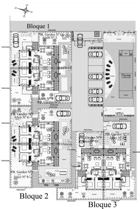
GENERAL PLAN
